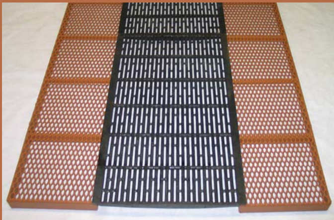
Dura Trac® Clearspan Creep Side in expanded metal with cast iron center
